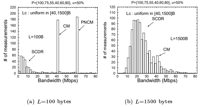
Figure 8: Small versus large probing size L .
