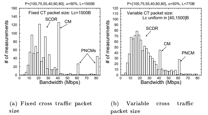
Figure 6: The effect of the cross traffic packet size L_c on the packet pair bandwidth distribution \mathcal{B} .
