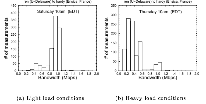
Figure 5: The effect of network load on the packet pair bandwidth distribution \mathcal{B} (measurements).
