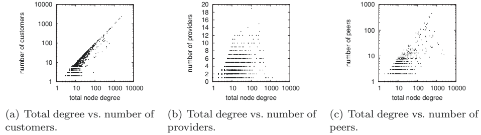
Fig. 8. Scatterplots demonstrating the diversity of annotation degrees and that total node degrees are agnostic with respect to annotations.
