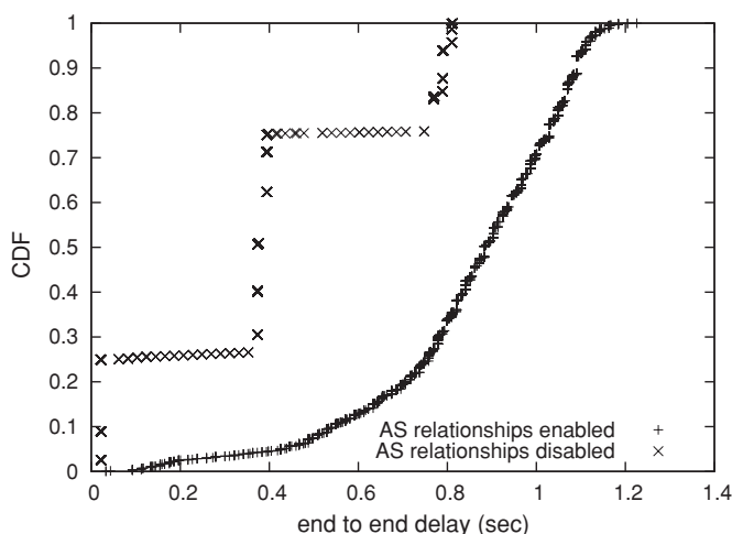
Fig. 2. CDF of e2e delay between traffic sources and destination.
