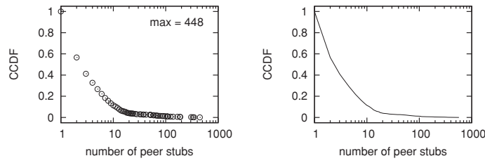
(a) Original distribution of 19,036 peer-degrees in the measured AS topology. (b) Continuous distribution approximating the original one.
