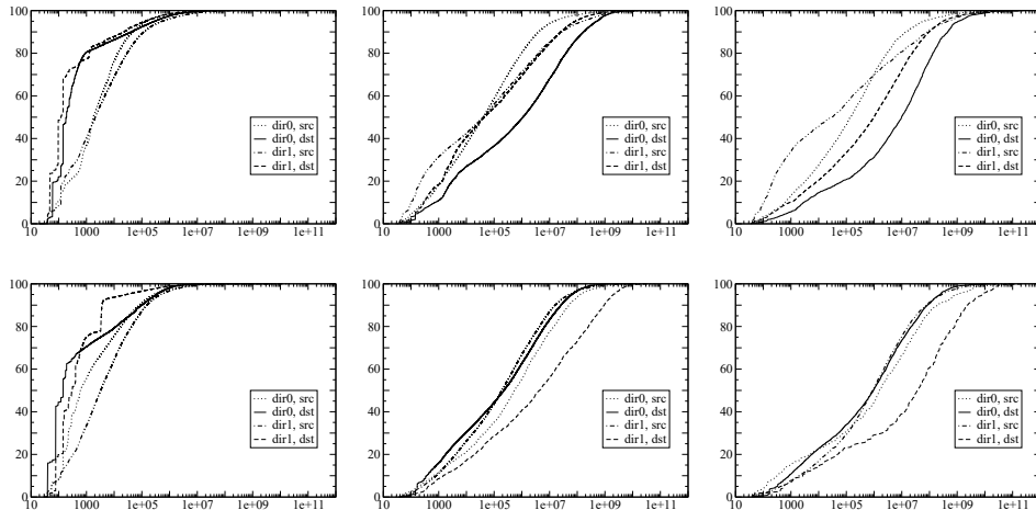
Fig. 5. IP addresses (left), prefixes (center) and ASes (right) as traffic sources (dotted lines) and sinks (solid and dashed lines). Object count cdfs over traffic volume (bytes per object). D04 (first row) and D09 (second).
