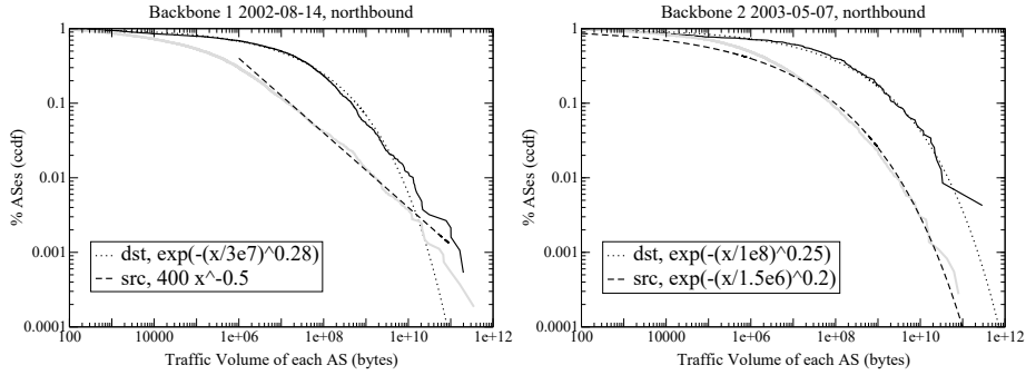
Fig. 4. Ccdf for source and destination bytes per AS. D04N (left), D09N (right).
