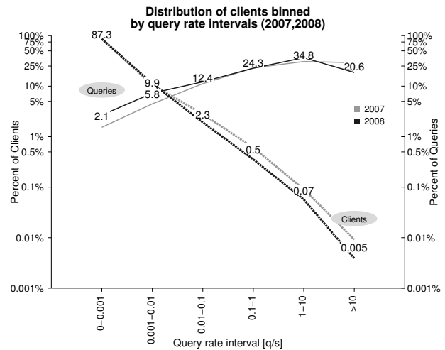
Figure 1: Distribution of clients by mean query rate in 2007 and 2008. The Y-axes use a log scale. This graph shows just a few clients (two rightmost categories) are responsible for more than 50% of the traffic at the observed root servers.
