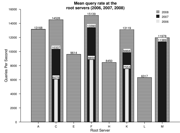
Figure 3: Average query rate observed at root servers participating in DITL 2006, 2007 and 2008. The solid light, dark, and hashed bars represent the average query rates in 2006, 2007, 2008, respectively.
