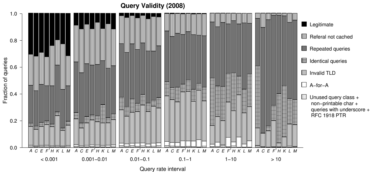
Figure 4: Validity of queries (2008). A strong correlation between the query rate and the amount of unwanted traffic could be observed. The amount of legitimate traffic (in black) reduces when the query rate increases.
