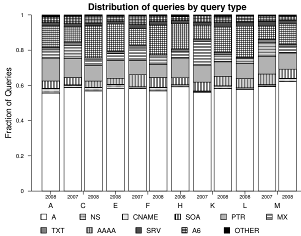
Figure 2: Distribution of queries by type. The distribution of query type shifted in 2008, including a significant increase in AAAA queries due to the addition of IPv6 glue records to six root servers in February 2008.
