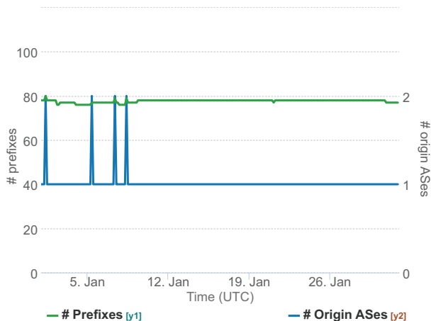
Figure 6: Monitoring of GARR (AS137) IP space using the pfxmonitor plugin. The green line reports the number of unique prefixes announced over time, the blue line reports the number of unique origin ASes that are currently announcing such prefixes. The spikes of the origin AS timeseries identify four hijack events in which AS 198596 announces part of the IP space belonging to AS137.
