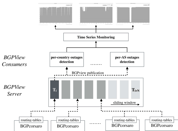
Figure 7: BGPStream framework deployment for live monitoring. For each collector, we run an instance of BGP-Corsaro with the routing-tables plugin, which maintains, in a hash table, the observable LocRIB of all the VPs of the collector. At the end of each time bin (e.g., 1 minute) each BGPcorsaro pushes its hash table to the BGPViewServer that, in turn, aggregates hash tables with the same timestamp into partial BGP views and publishes them once they become complete. Such data can be further processed by the BGPViewConsumers, which handle the results of their computation to a Time Series Monitoring system.
