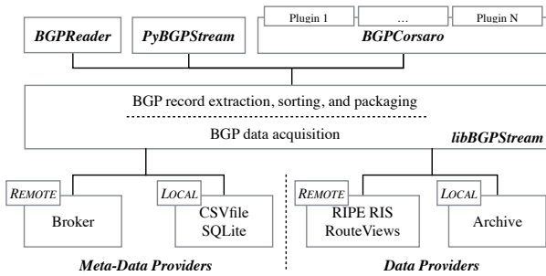
Figure 2: BGPStream framework overview. The BGPStream framework is organized in three layers. From bottom up, these are: data and meta-data access, records extraction and packaging ( libBGPStream ), and record processing ( BGPReader , PyBGPStream , BGPCorsaro ).
