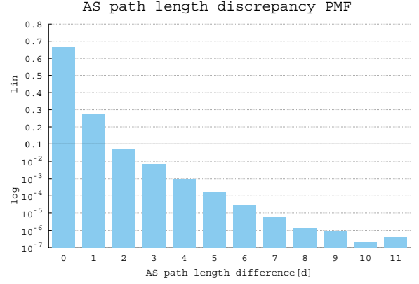
Figure 5: The extent of AS paths inflation. Probability mass function of the difference in length between the shortest AS path observed in BGP and in the undirected graph for the same \langle VP, origin \rangle pairs. The y axis is logarithmic up to 10^{-1} and then linear. Almost 70% of the paths observed do not experience inflation ( x = 0 ).
