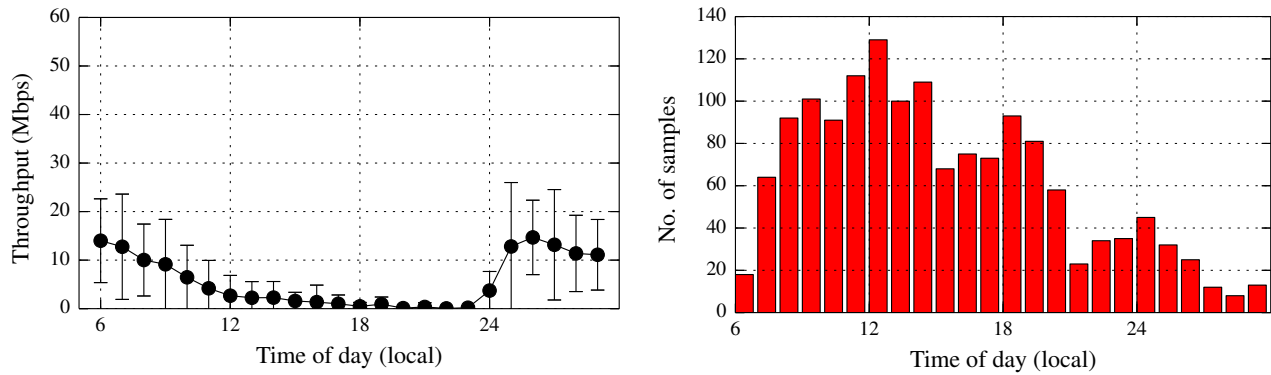
(a) GTT server in Atlanta to AT&T customers. (May 2015)
