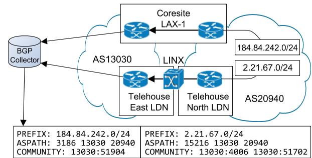
Figure 4: Inferring physical locations from BGP Communities.
