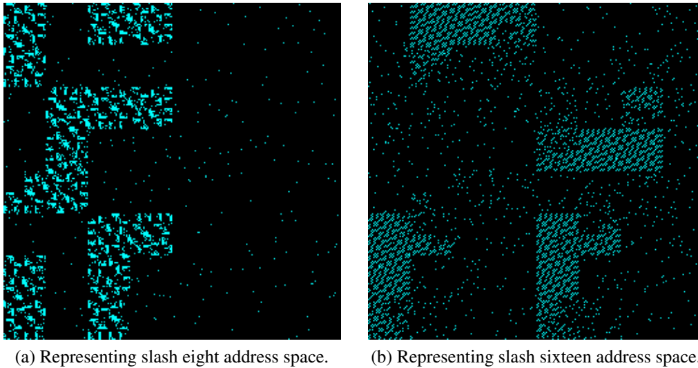
Figure 3.10: Heatmap of destination IPs generated by Hilbert curve in SYNRENT Phase 2. a) Each pixel represents /16 address block in the UCSD-NTs address space. b) Each pixel represents /24 address block in the UCSD-NT’s address space.
