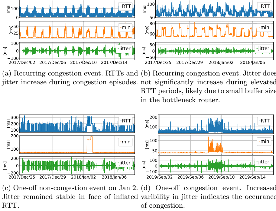
Fig. 1. Typical examples of network events. The raw timeseries (top figures) is the raw RTT data with 5-minute resolution. We aggregate the raw data into 15-minute buckets with the minimum function to filter noise (middle figures). We compute jitter using the 15-minute aggregated data to quantify variability in RTTs (bottom figures).
