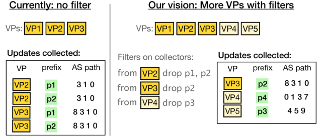
(b) Our overshoot-and-discard approach (right) collects fewer updates from more useful VPs, which better reveals routing events compared to current approach (left).
