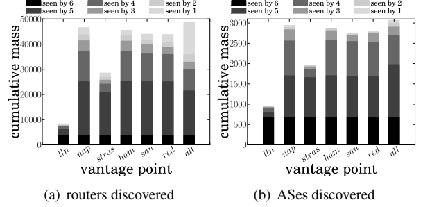
Figure 7: Vantage point utility
