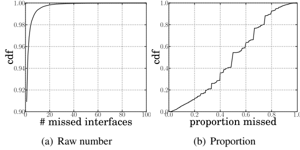
Figure 8: Interfaces missed for responding routers
