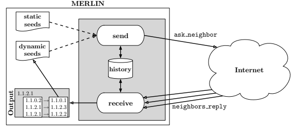
Figure 2: MERLIN architecture
