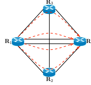
Figure 3: Reprobing risk on R_4 - 4 probes may reach it
