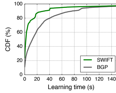
Figure 8: SWIFT quickly learns about remote outages. In 2 (resp. 9) seconds, SWIFT learns more than 50% (resp. 75%) of the withdrawals, BGP needs 13 seconds (resp. 32 seconds).
