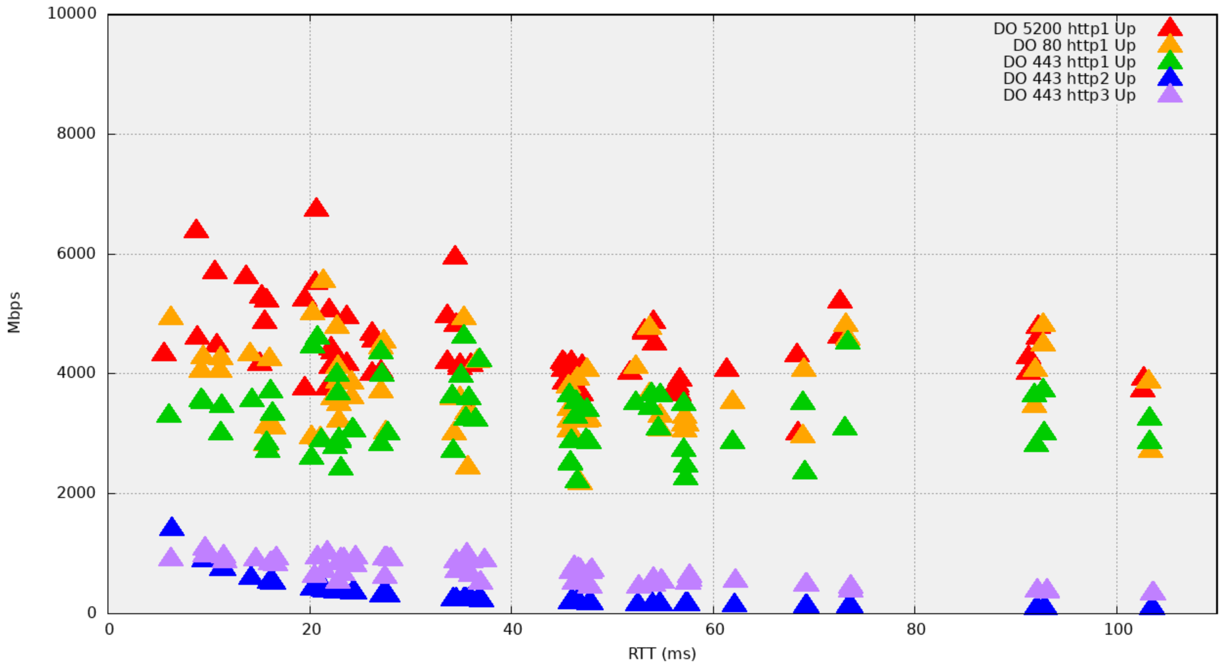
DREN Internal (DO) Upload
