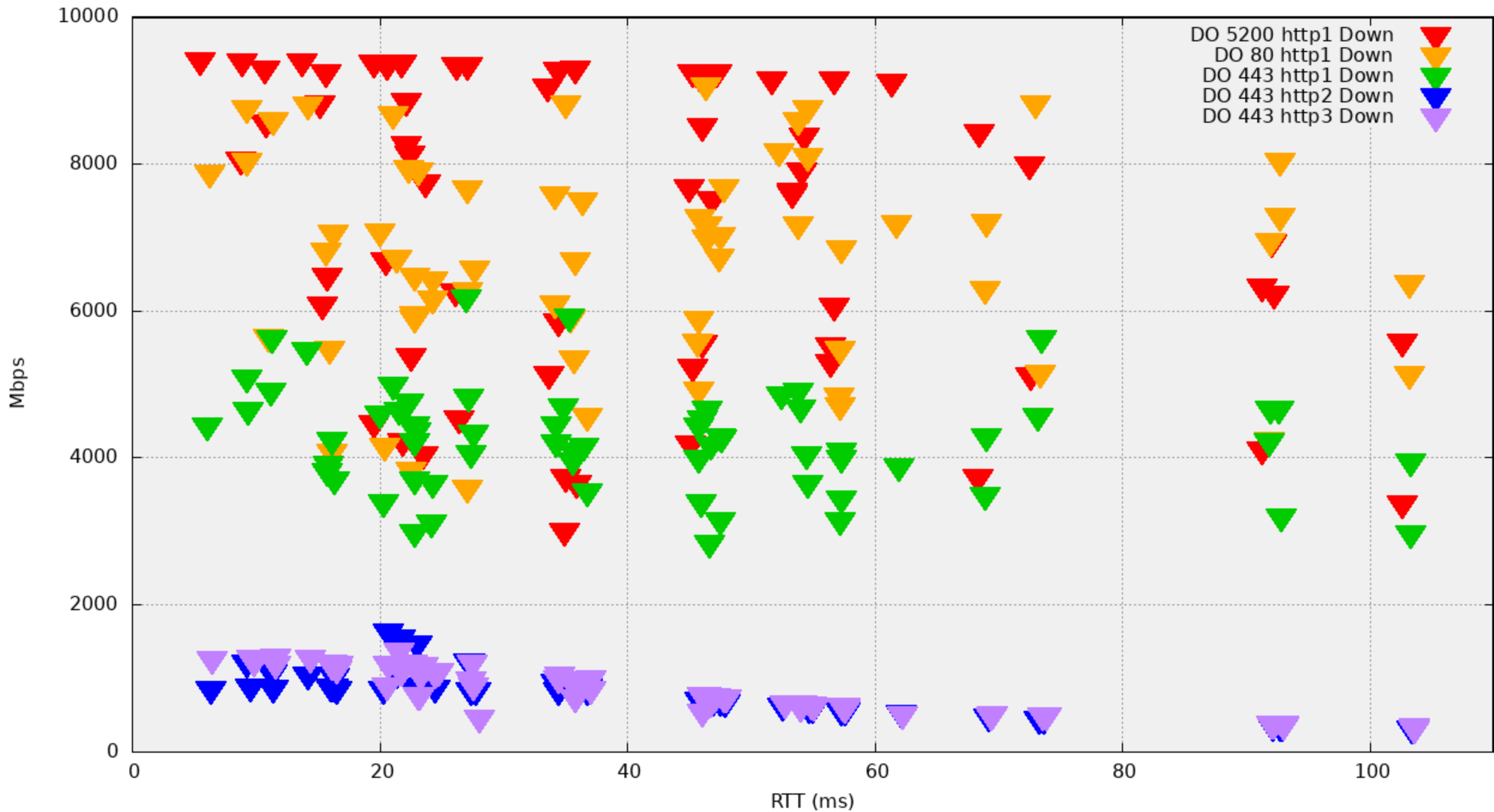
DREN Internal (DO) Download
