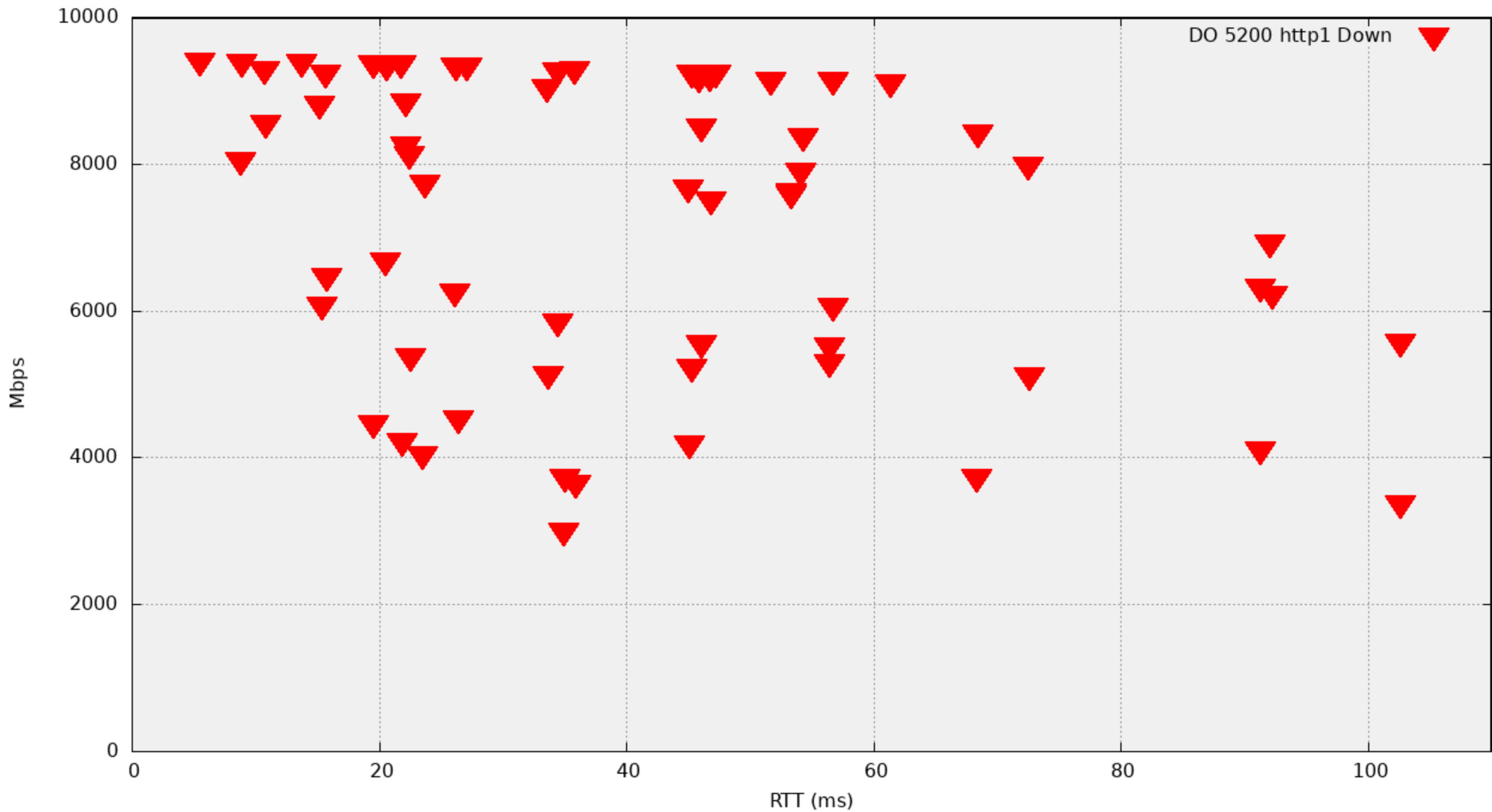
DREN Internal (DO) Downloads, port 5200 http1
